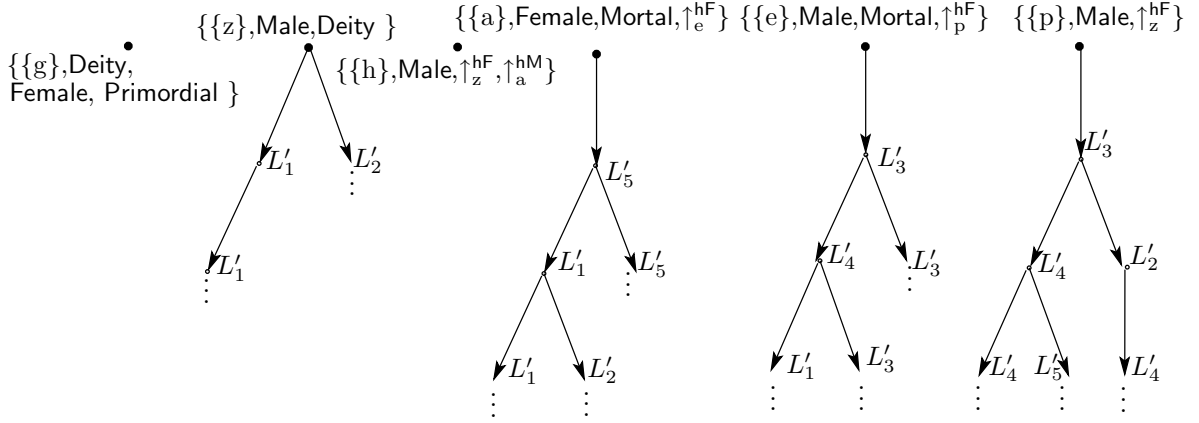
Figure 3.3: The forest encoding of the canonical model in Figure 3.2
