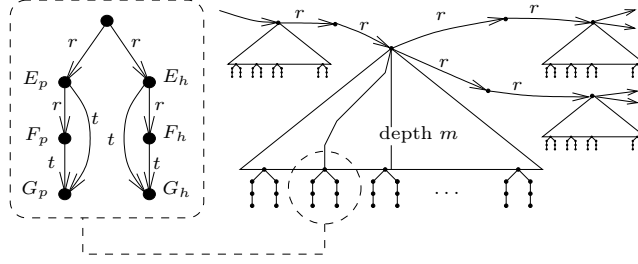
Figure 7.9: The structure of models.
