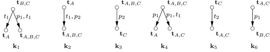
Figure 7.1: Example set of knots
