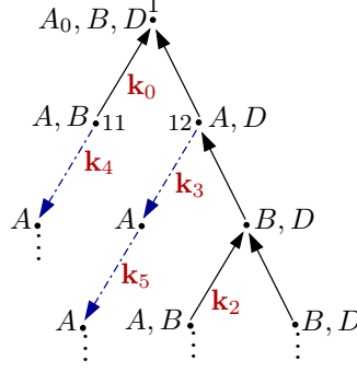
Figure 6.5: A canonical model \mathcal{I}_a for \mathcal{K}_a
