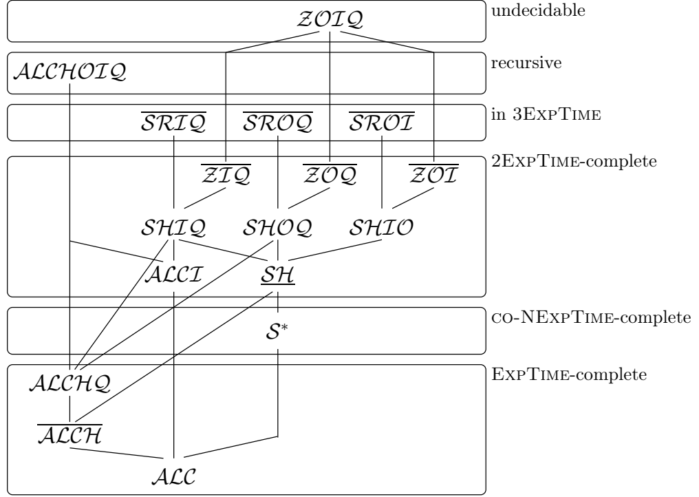
Figure 8.1: The complexity of query answering in expressive DLs. For the overlined/underlined logics, the upper/lower bound was shown in this thesis.
