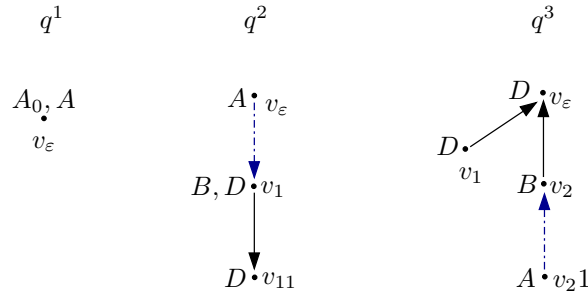
Figure 6.7: A set Q_a of tree-shaped queries
