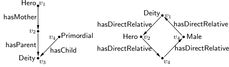
Figure 2.7: The query graphs of q_3^{theo} and q_4^{theo}
