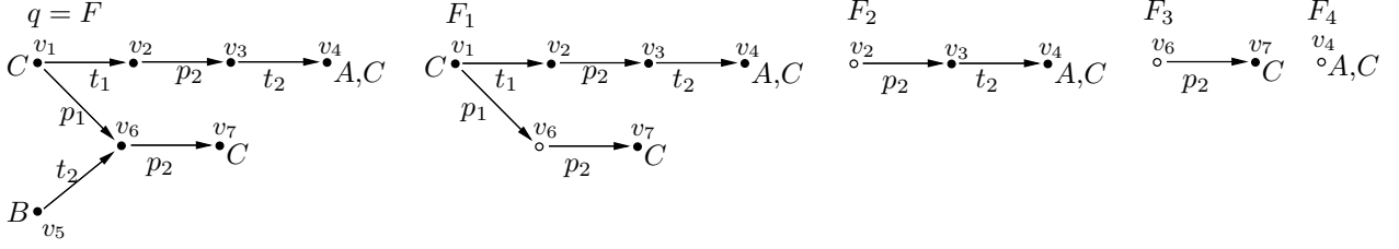
Figure 7.3: An example query and some of its f-subqueries
