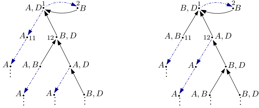
Figure 6.1: Two canonical models \mathcal{I}_1 and \mathcal{I}_2 for \mathcal{K}_1
