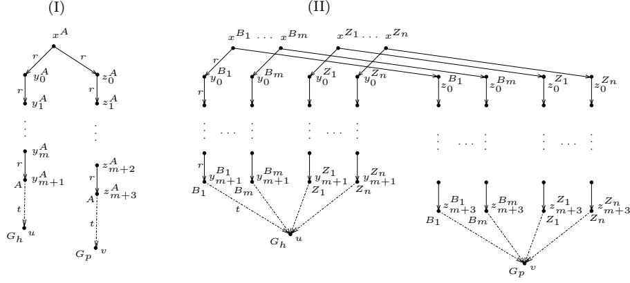
Figure 7.10: The basic query q(A, u, v) and the final query q_{\mathcal{M}, w} .
