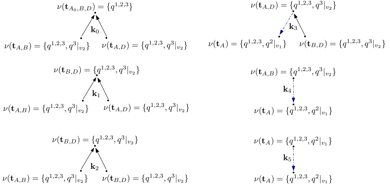
Figure 6.8: A set \mathbb{K}'_a of Q_a avoiding knots
