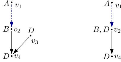
Figure 6.11: The query q_1 and its fork-elimination \text{FE}(q_1)
