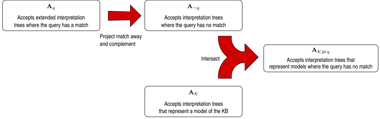
Figure 4.3: Overview of the automata algorithm for Query Entailment
