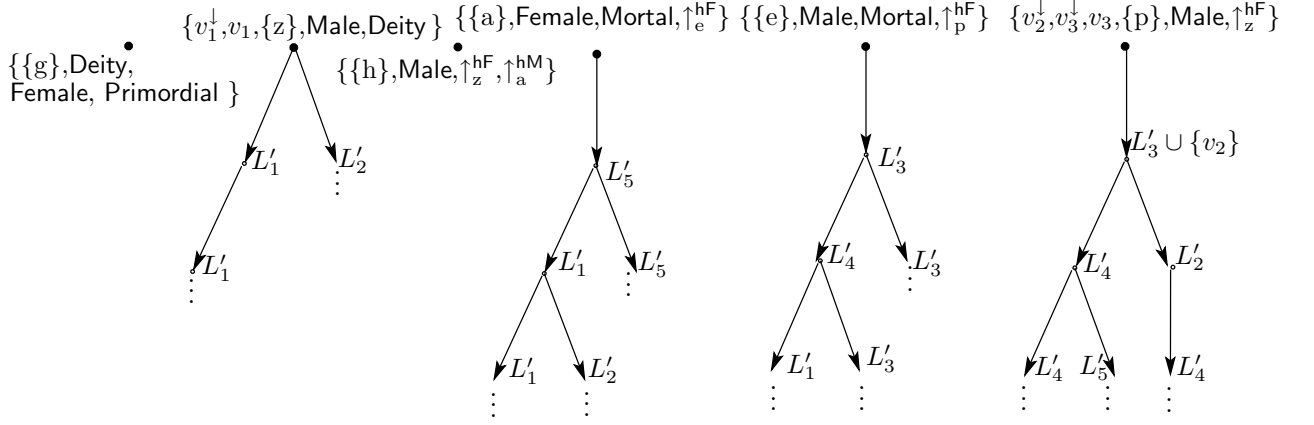
Figure 4.2: The forest representation of an extended interpretation
