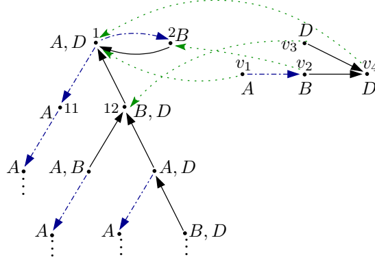
Figure 6.3: A match for q_1 in \mathcal{I}_1
