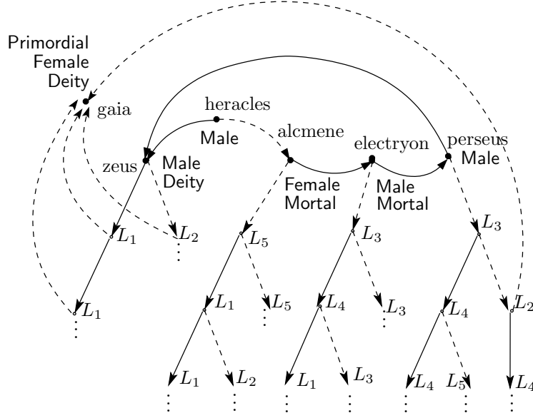
Figure 3.2: A canonical \mathcal{I}_g model for \mathcal{K}_g
