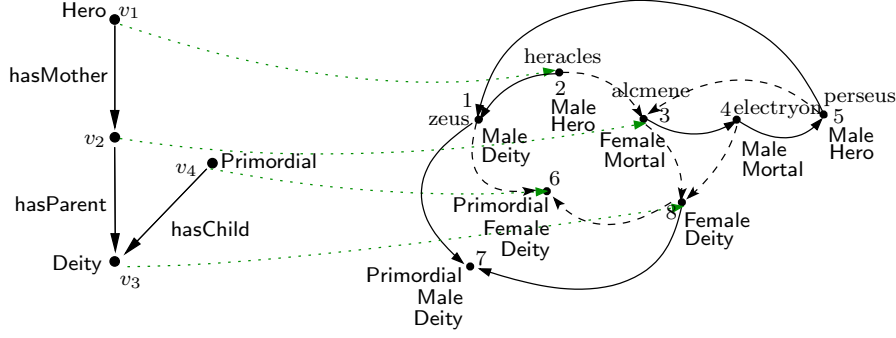
Figure 2.8: An example of a query match for q_3^{theo} in \mathcal{I}_1
