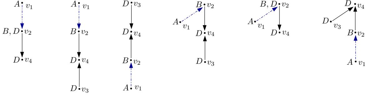
Figure 6.10: Some tree rewritings of q_1
