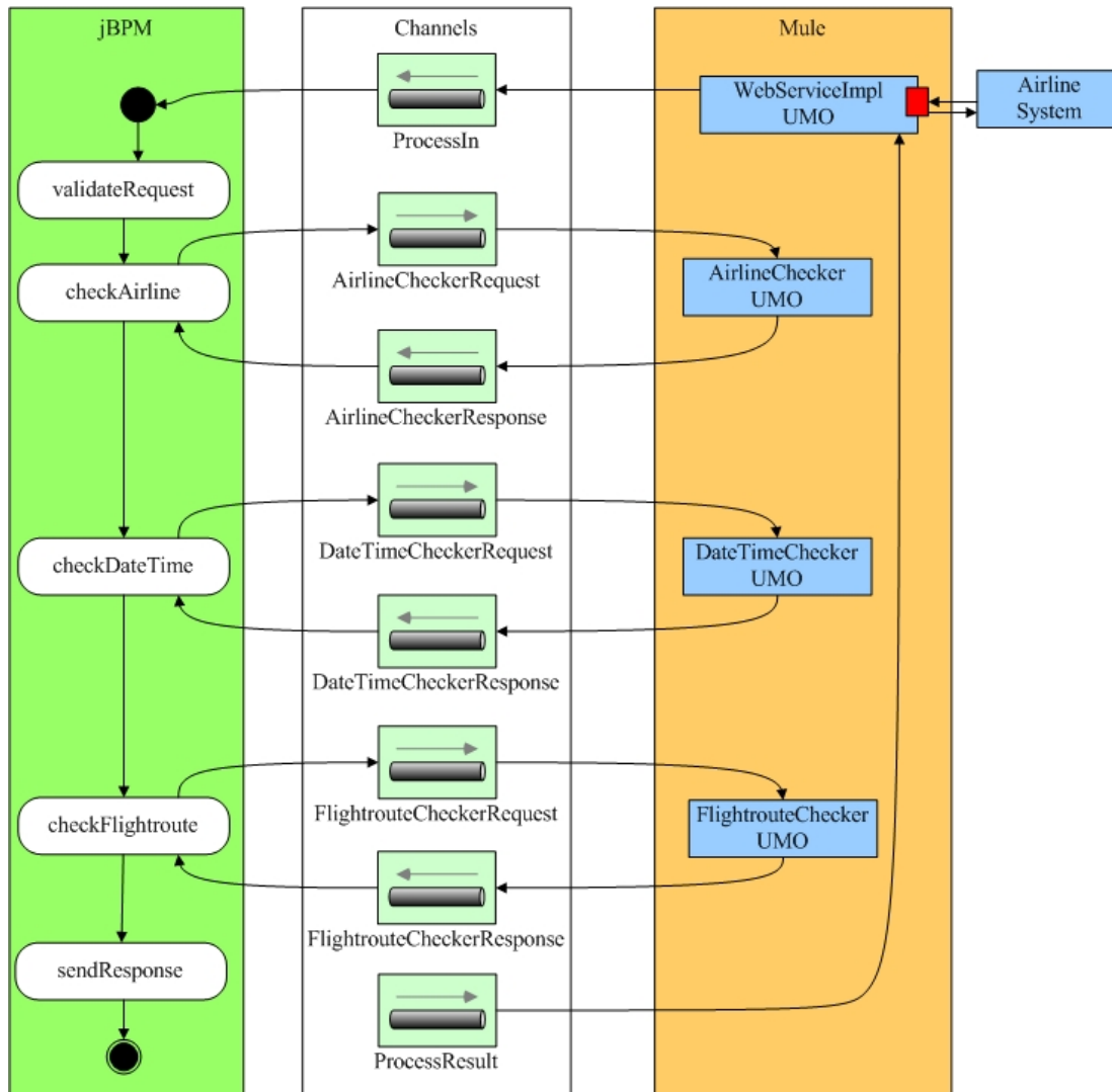
Figure 5.1: Cooperation between Mule and jBPM engine
