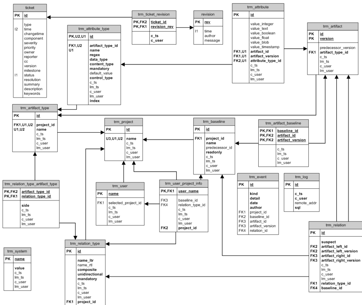
Figure 14: Excerpt of the TreqPro database schema
