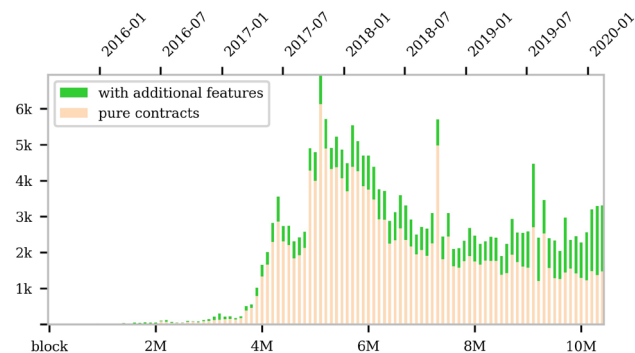
Fig. 4 Deployment of ERC-20 token contracts, divided into pure (peach) and non-pure (green) tokens. The lower horizontal axis indicates the Ethereum blocks, while the upper axis shows the corresponding dates. Each bar represents a bin of 100,000 blocks corresponding roughly to 2 weeks (color figure online)
