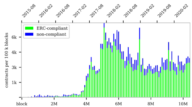
Fig. 3 Deployment of all token contracts, differentiated into ERC-compliant ones in green and non-compliant ones in blue. The lower horizontal axis indicates the Ethereum blocks, while the upper axis shows the corresponding dates. Each bar represents a bin of 100,000 blocks corresponding roughly to 2 weeks (color figure online)
