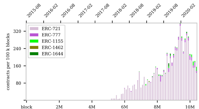
Fig. 2 Creation of ERC-compliant token contracts other than ERC-20. The lower horizontal axis indicates the Ethereum blocks, while the upper axis shows the corresponding dates. Each bar represents a bin of 100,000 blocks (corresponding roughly to 2 weeks)
