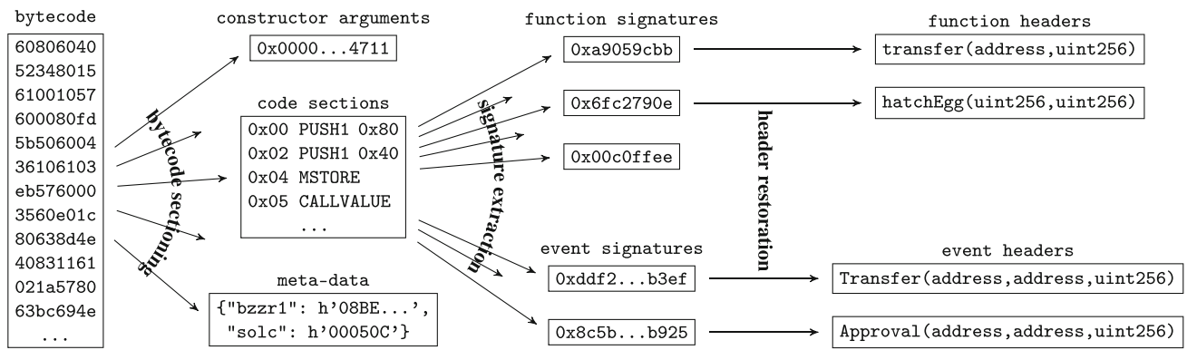
Fig. 1 Interface reconstruction: after decomposing the bytecode into code sections, data and meta-data, we extract the function and event signatures from the first code segment. Using dictionaries with known headers, we are able to restore most function and event headers
