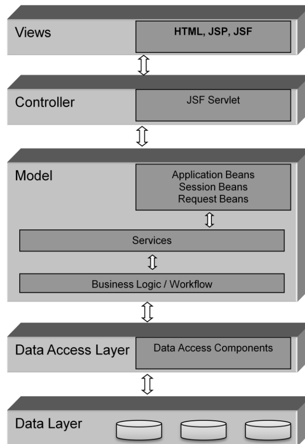
Diagram 56: Model-View-Control - Architecture
