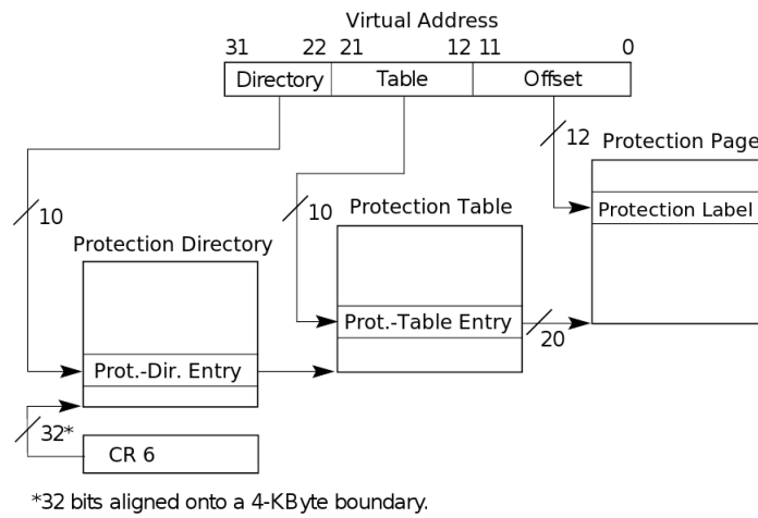
Figure 3.1: Protection hierarchy.
