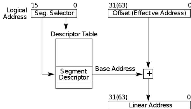
Figure 2.1: Logical to linear memory translation. [23]
