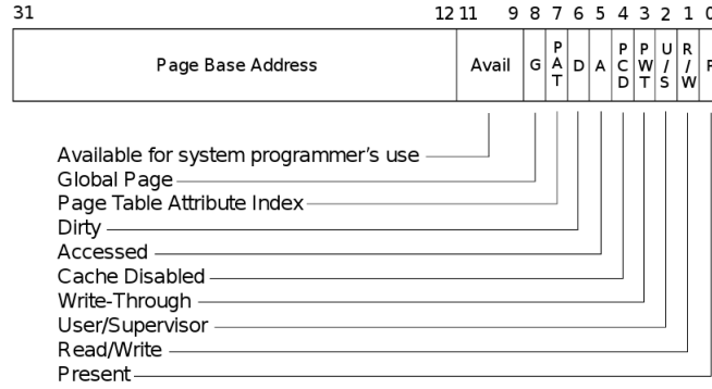
Figure 2.4: Page-table entry of a 4 kibibyte page. [23]
