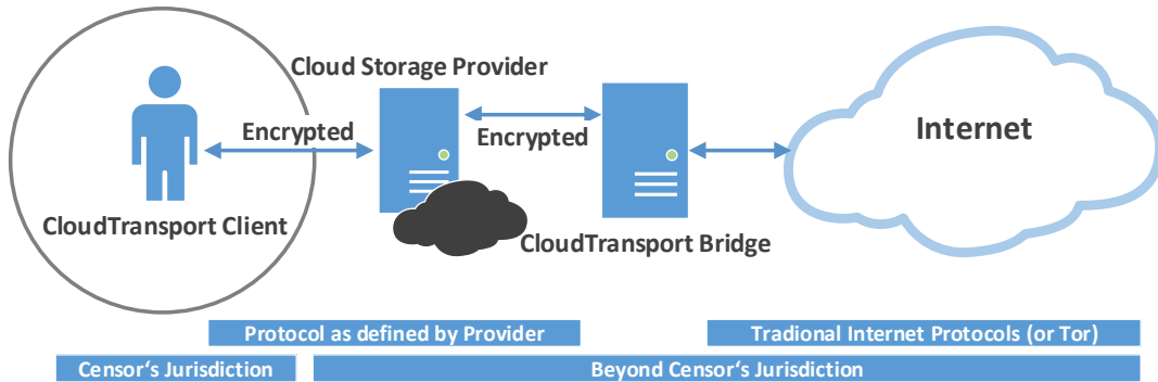
Figure 3.9: CloudTransport: Architecture
