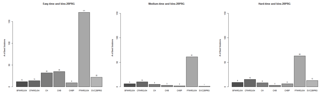
Figure 6.10: Number of instances for the 2BPRG case on which the algorithms obtain the best solution for the hardness subgroups using the main criteria
