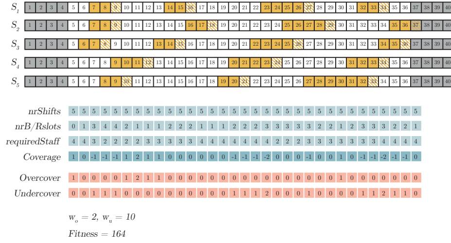
Figure 3.2: A graphical example of the calculation of Coverage , Overcover , Undercover and Fitness of five shifts. First nrB/Rslots needs to be determined by accumulating all b- and r-slots for each timeslot. Then the coverage is calculated by subtracting nrB/Rslots and requiredStaff from nrShifts . Finally the over- and undercover is derived. Setting the weights w_o to 2 and w_u to 10, the resulting fitness amounts 216.
