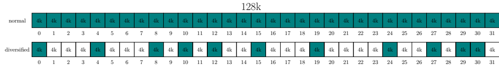
Figure 5.1: Witout PAGE SACRIFICE all blocks are deterministically allocated and used. With PAGE SACRIFICE not all pages are used, but their positioning is unpredictable in advance.
