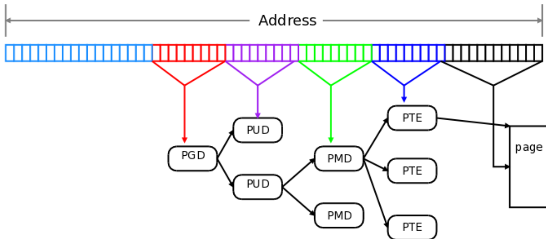
Figure 2.6: Four-level page table hierarchy of Linux for a x86_64 processor. Graphic by Jonathan Corbet https://lwn.net/Articles/717293/
