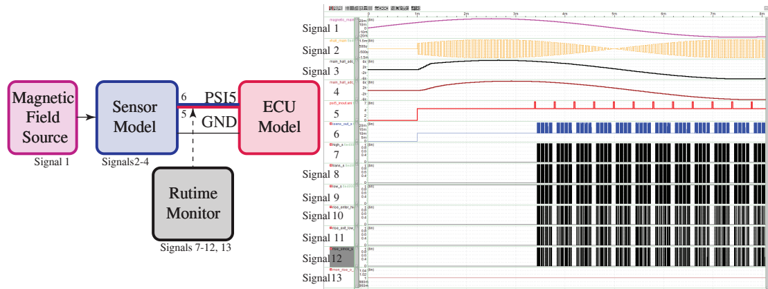
Figure 7.4: The runtime monitor in simulation: setup and results
