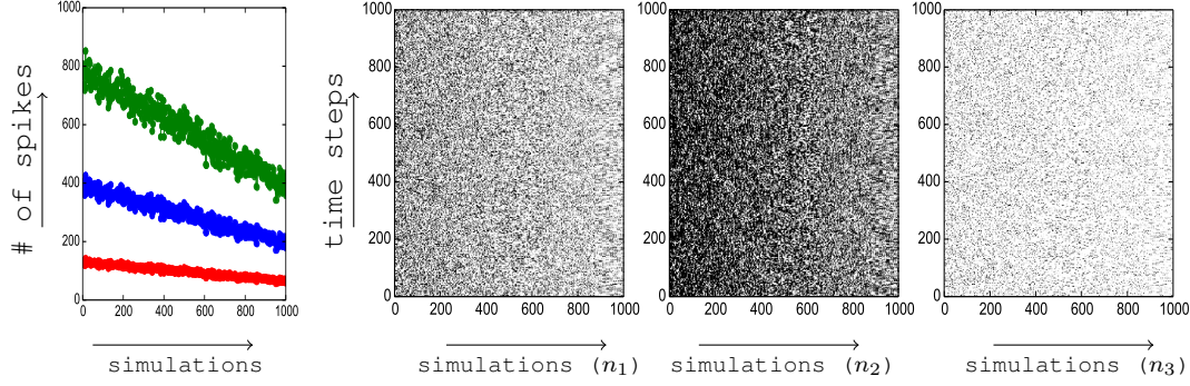
Figure 6.5: Constant multiplication and division of the spike rates with the TrueNorth model: 2 \cdot \text{blue} = \text{green} , \frac{1}{3} \cdot \text{blue} = \text{red} ( n_1 – blue; n_2 – green; n_3 – red)
