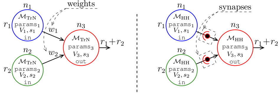
Figure 6.2: Neural models for computations on spike rates
