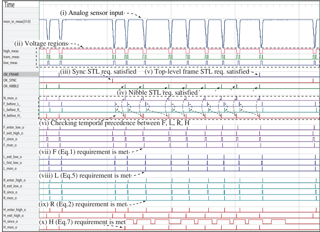
Figure 8.10: Runtime monitoring of the STL requirements
