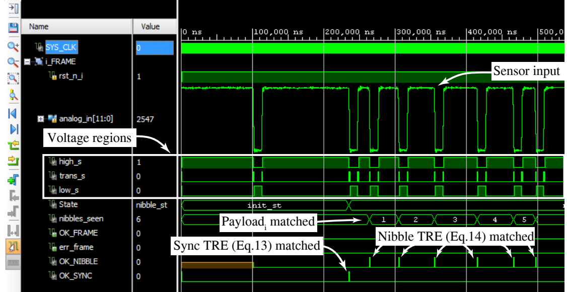
Figure 8.8: Runtime TRE monitoring: Vivado functional simulation
