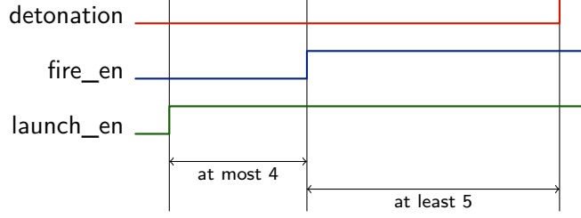
Figure 5.4: Missile timing property specification
