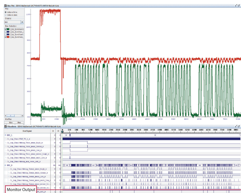
Figure 7.6: Runtime Monitor in Hardware: Chip Scope Results
