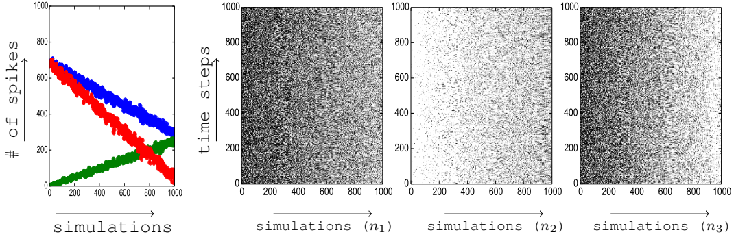
Figure 6.7: Subtraction in the spike rates with the TrueNorth model: blue – green = red ( n_1 – blue; n_2 – green; n_3 – red).
