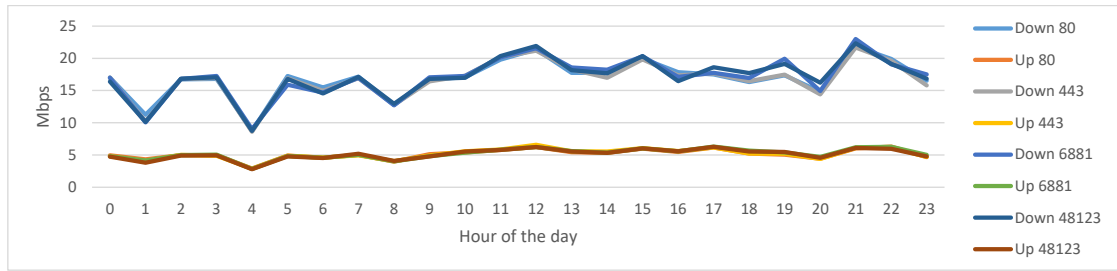
Figure 4.8: Test speed on different ports depending on the UTC hour of day for A1 LTE
