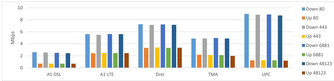
Figure 4.6: Test speeds (Mbps) on different ports for the tested ISPs, corresponding to Table 4.7
