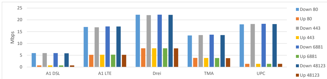
Figure 4.7: Test speeds (Mbps) on different ports for the tested ISPs, corresponding to Table 4.8
