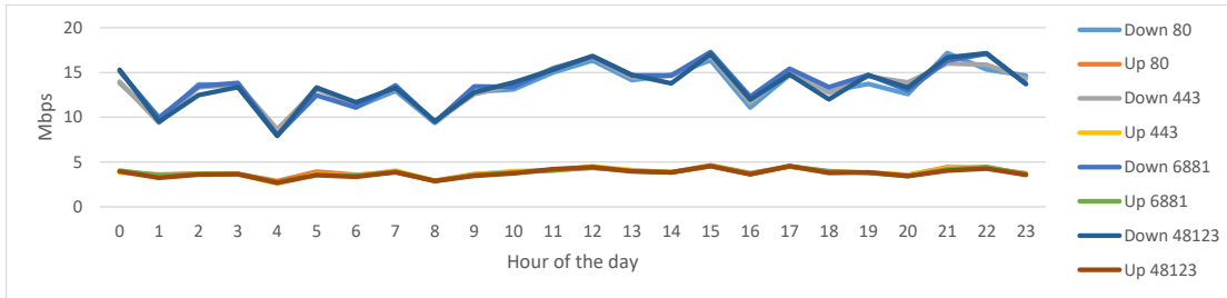
Figure 4.12: Test speeds on different ports depending on the UTC hour of day for T-Mobile
