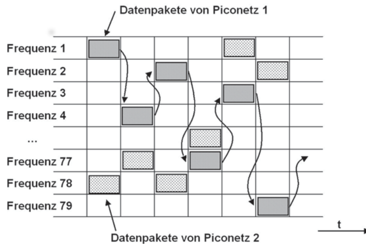
Abbildung 3.5: Frequency Hopping [PROT2012, S.360]
