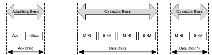
Abbildung 3.8: Connection Events [BLUESTD, S.172]
