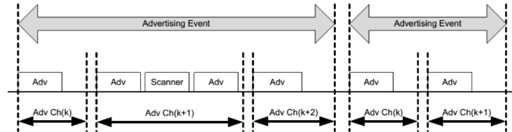
Abbildung 3.7: Advertising Events [BLUESTD, S.172]
