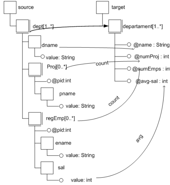
Figure 4.11: A CLIP mapping with aggregates (adapted from [37, Figure 9])
